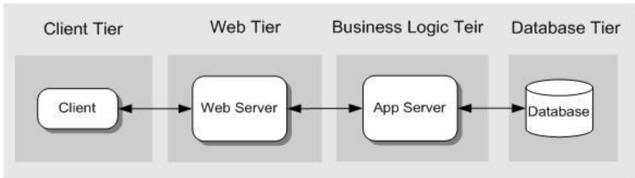
Fig: An example of N-tier Architecture
