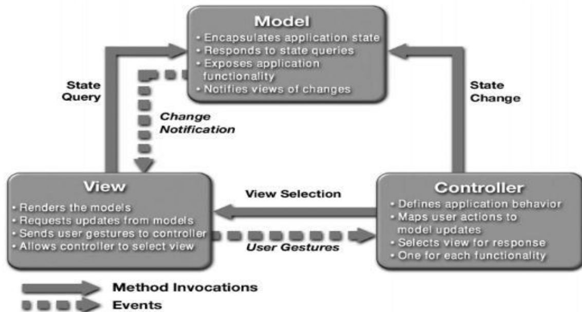
Fig: Summary of relationship between Model, View and Controller
